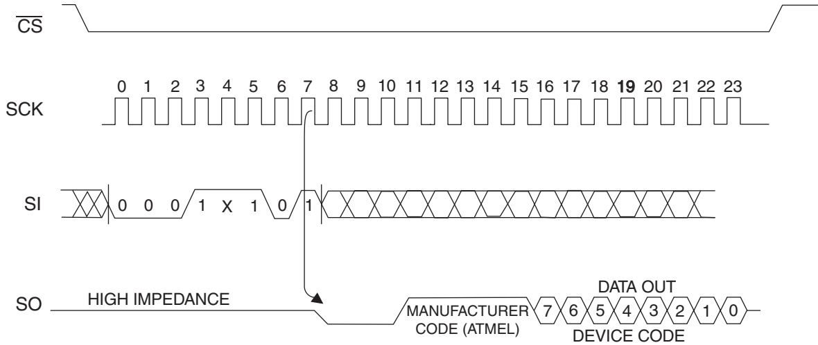
Figure 13. RDID Timing
