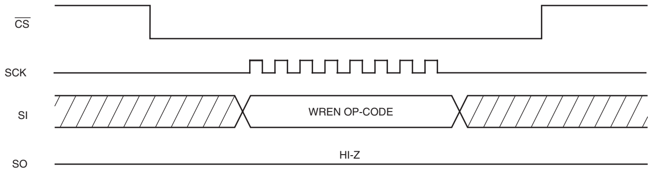
Figure 4. WREN Timing
