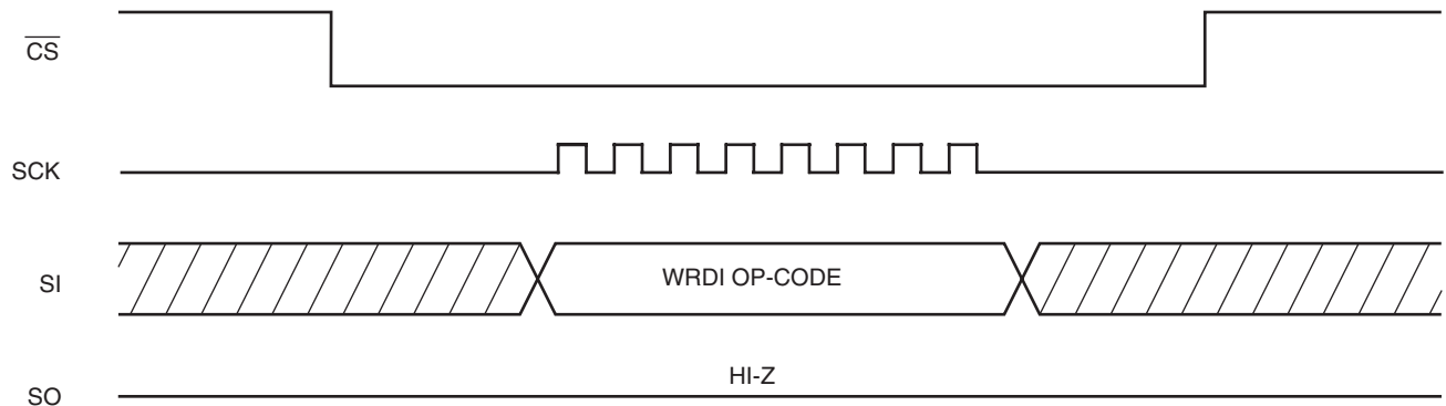
Figure 5. WRDI Timing
